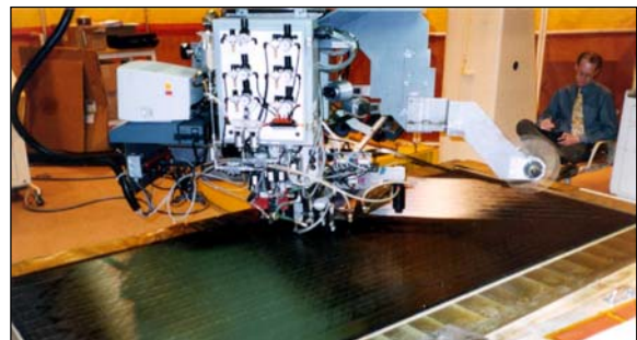
Figure 1 Thermoplastic automated tape placement is used to accurately consolidate deposit a 45° ply in place.
